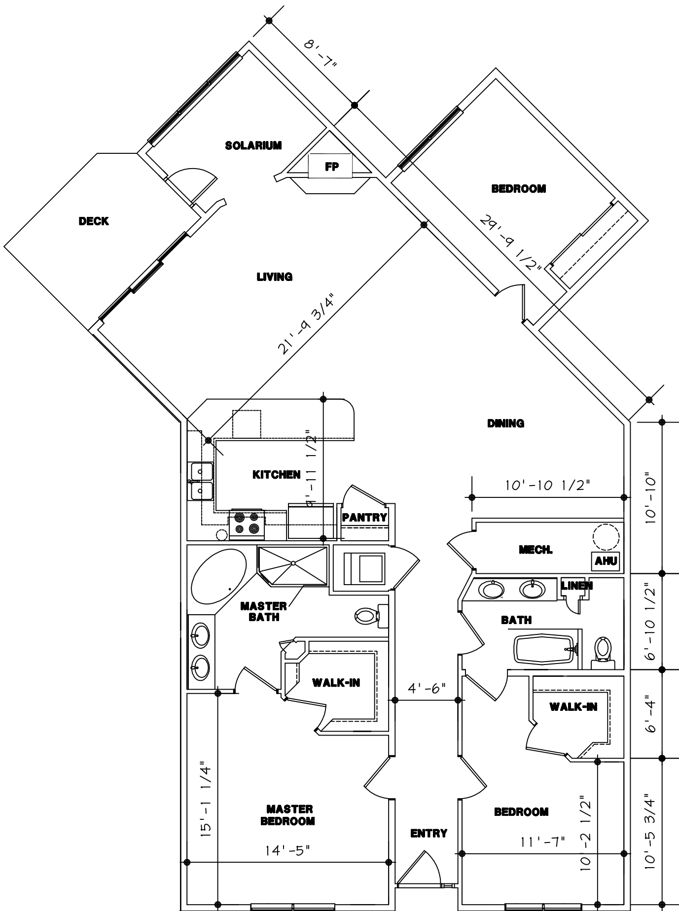
THREE BEDROOM - TWO BATH UNIT
